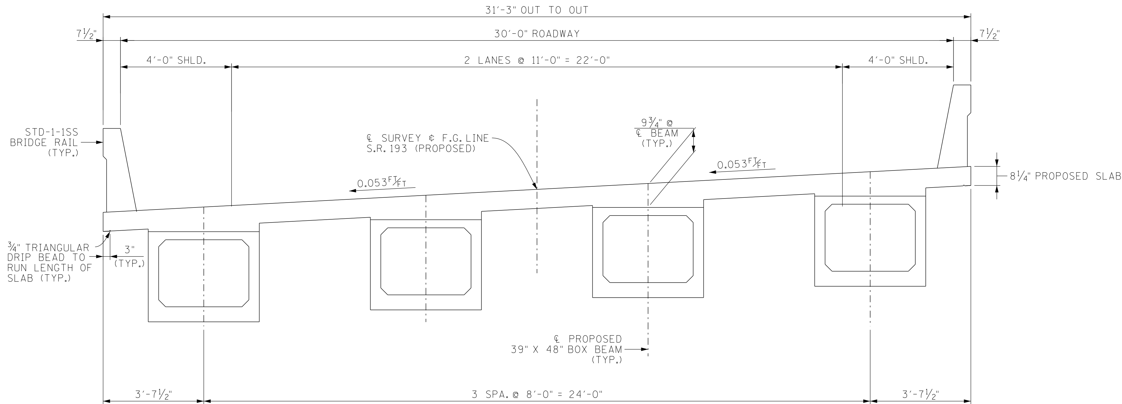
TYPICAL SECTION - PROPOSED (LOOKING FORWARD ON SURVEY)
